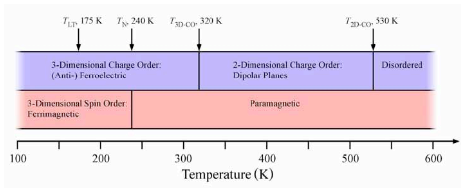
Figure 5.10: Phase diagram of \text{LuFe}_2\text{O}_4 , showing the electronic, magnetic and structural transitions.
