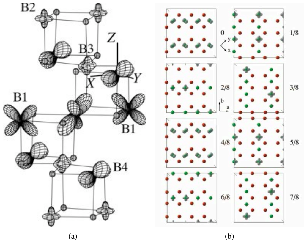
Figure 2.6: (a) Charge and orbital structure predicted by Leonov et al. The extension along the c -axis shown represents one cubic unit cell length, which is half as long as the P2/c and Cc unit cell. Figure from reference 68. (b) Orbital structure predicted in the t_{2g} band for the Cc structure by Jeng et al. The red and green spheres represent oxygen and iron atoms respectively. The crystallographic ( Cc ) axes are given by a and b , while cross-sections are shown along the c -axis. Reprinted figures with permission from references 68 and 67 respectively. Copyright 2004 and 2006 by the American Physical Society.
