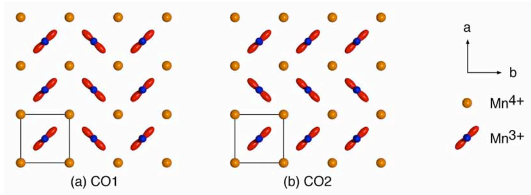
Figure 4.5: The direction of the orbital stripes in the (a) CO1 and (b) CO2 phases in \text{Pr}(\text{Sr}_{0.1}\text{Ca}_{0.9})_2\text{Mn}_2\text{O}_7 . The solid line shows the high temperature crystallographic unit cell.
