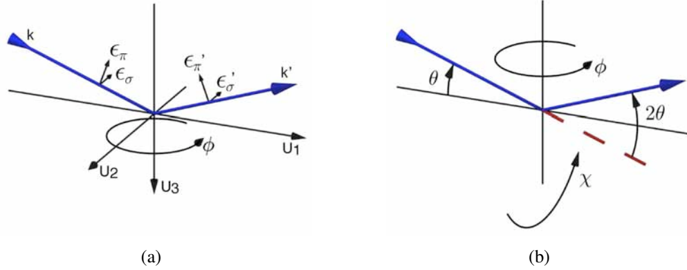
Figure 1.9: The scattering geometry indicating (a) the incoming and outgoing channels, as well as the U basis vectors defined by this set-up [41] and (b) the motor movements. In the figure and the text, a prime signifies the scattered component.
