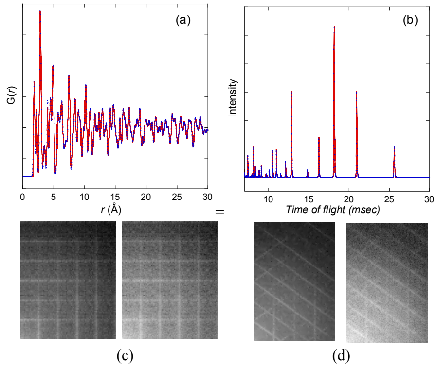
Figure A4.2: Results of a simultaneous fit of the neutron PDF and Bragg profile and electron diffuse scattering (two sections). (a, b) Experimental (blue) and calculated (red) neutron PDF (a) and Bragg profile (b). Experimental (left) and calculated (right) electron diffuse scattering patterns in the (130) (c) and (114) (d) sections of reciprocal space.
