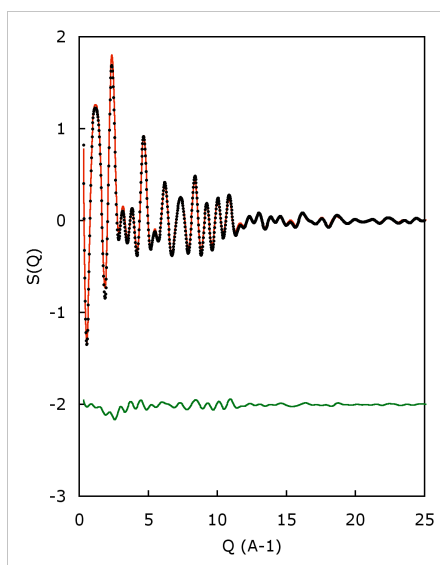
Figure 8: A typical equilibrium RMC fit to neutron scattering data for MnO.
