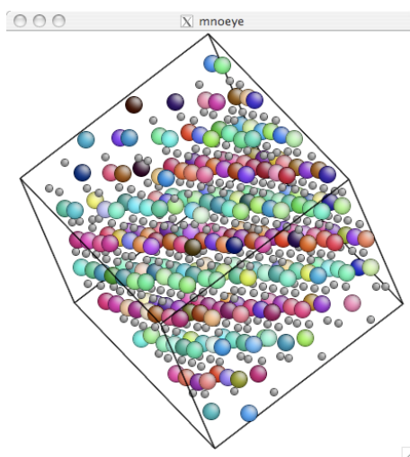
Figure 9: A typical RMC equilibrium configuration as seen in ATOMEYE.
