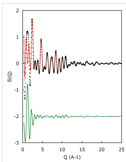
Figure 7: Initial RMC fit to neutron scattering data for MnO. Data are shown as solid points, the RMC fit as a red line, and the difference (data–fit) shown as a green line, shifted by 2 units.
