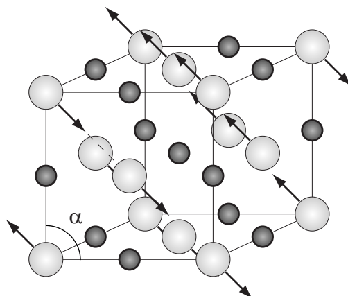
Figure 5: The antiferromagnetic structure of MnO: Mn and O atoms are shown as large light-grey and small dark-grey spheres, respectively.
