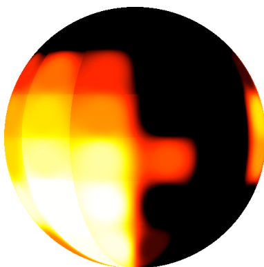
Figure 10: A typical spherical spin distribution (black = low probability; white = high probability). The view is taken looking down [100] with the [010] axis to the right hand side, and the [001] axis towards the top of the figure. In this particular case, alignment appears to be approximately parallel (and antiparallel) to [112] .
