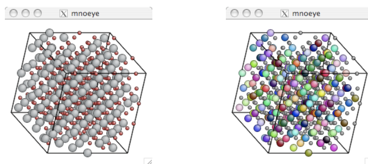
Figure 6: The RMC starting configuration as seen in ATOMEYE, using default colouring (left) and with Mn atoms coloured by the initial spin directions (right).
