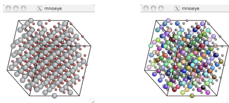
Figure 2: The RMC starting configuration as seen in ATOMEYE, using default colouring (left) and with Mn atoms coloured by the initial spin directions (right).
