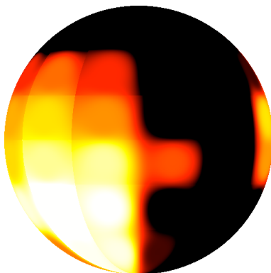
Figure 6: A typical spherical spin distribution (black = low probability; white = high probability). The view is taken looking down [100] with the [010] axis to the right hand side, and the [001] axis towards the top of the figure. In this particular case, alignment appears to be approximately parallel (and antiparallel) to [112] .
