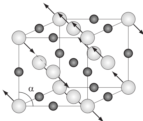
Figure 1: The antiferromagnetic structure of MnO: Mn and O atoms are shown as large light-grey and small dark-grey spheres, respectively.
