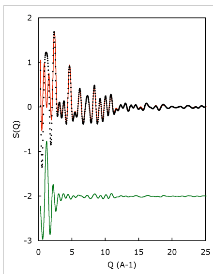
Figure 3: Initial RMC fit to neutron scattering data for MnO. Data are shown as solid points, the RMC fit as a red line, and the difference (data–fit) shown as a green line, shifted by 2 units.
