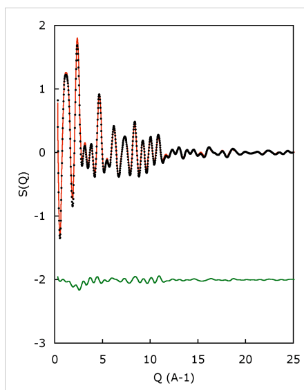
Figure 4: A typical equilibrium RMC fit to neutron scattering data for MnO.
