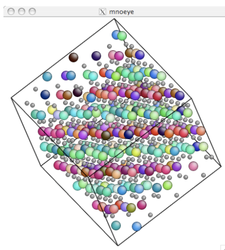
Figure 5: A typical RMC equilibrium configuration as seen in ATOMEYE.
